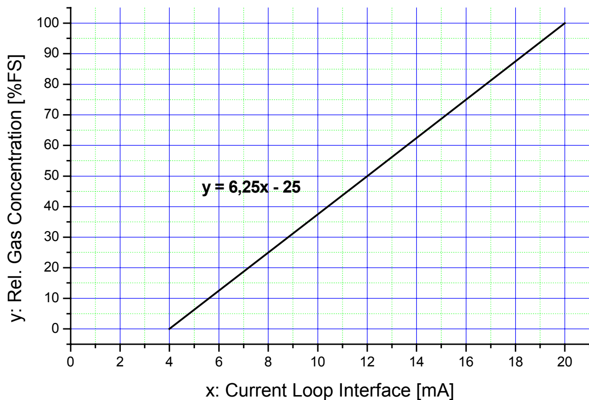
Transfer Function
