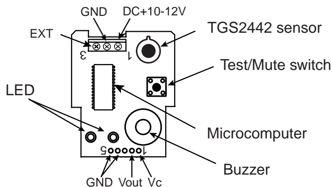
Figure 1 - COM2442 configuration
