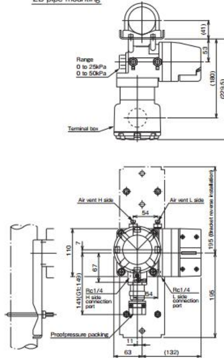
2B pipe mounting
