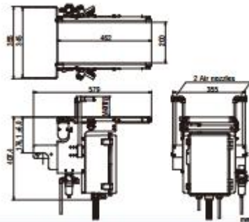
AD-4984-2046 External Dimensions
