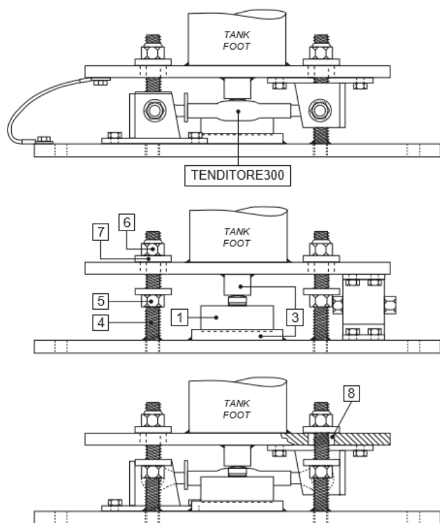
Application example with compression load cells
