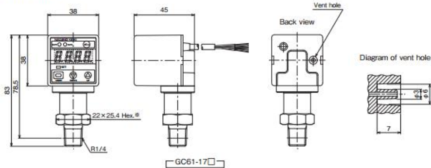
Horizontal mounting
