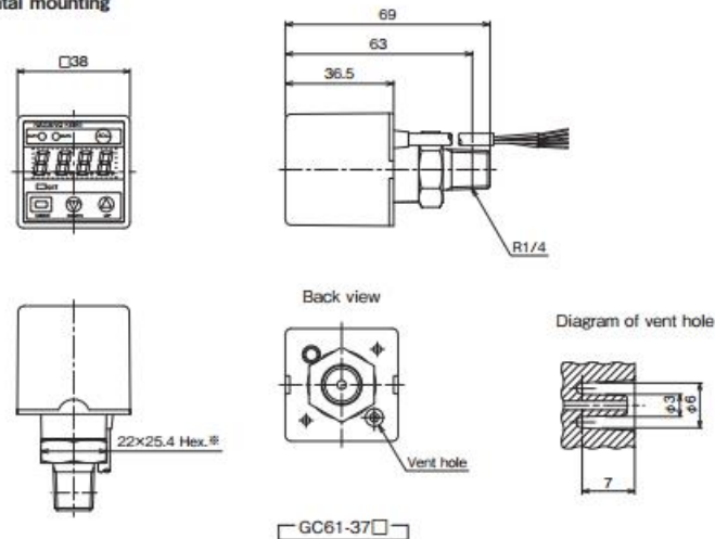
Horizontal mounting
