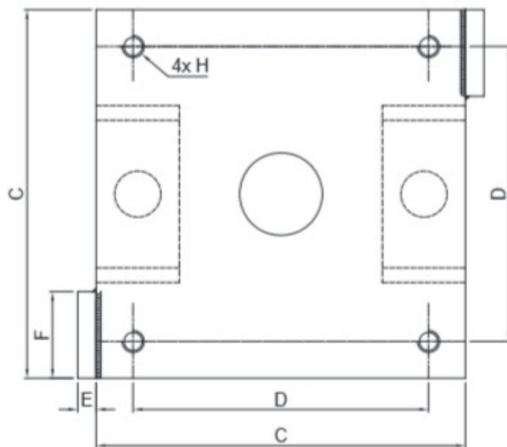
Lower plate
