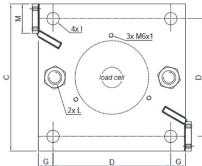
Lower plate
